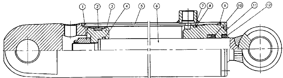
Cylinder 80/40-180
